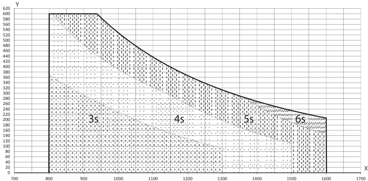
Diagram showing the use of Powerturn with opening times of up to 90° door opening angle
