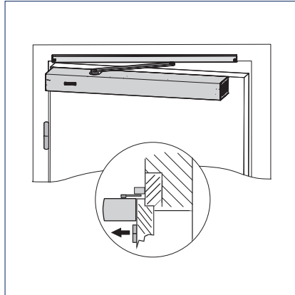
Door leaf installation with guide rail / roller guide rail
