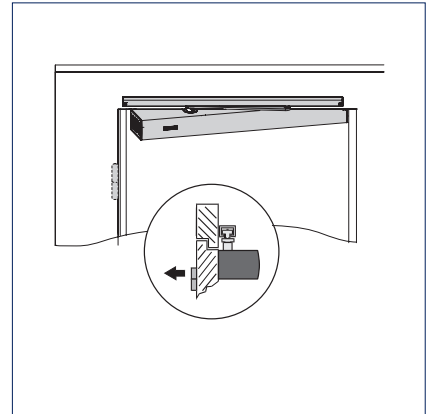
Door leaf installation with guide rail / roller guide rail
