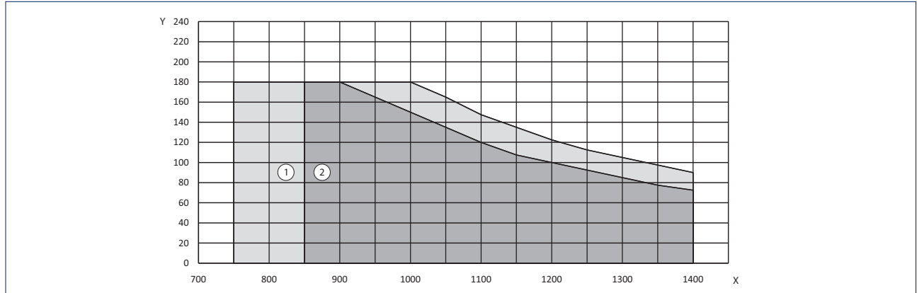
Slimdrive EMD
