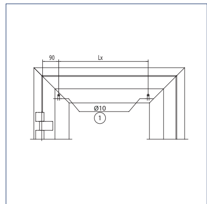
Safety sensor drill hole distances hinge side
