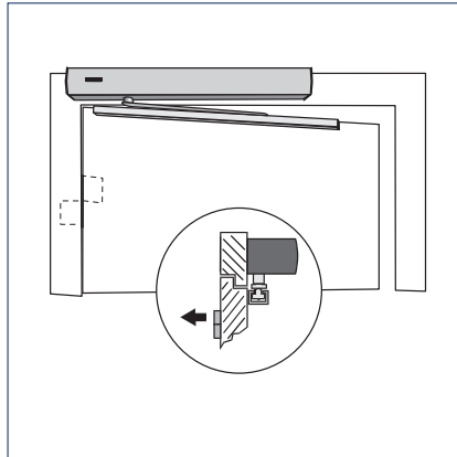
Transom installation with guide rail / roller guide rail
